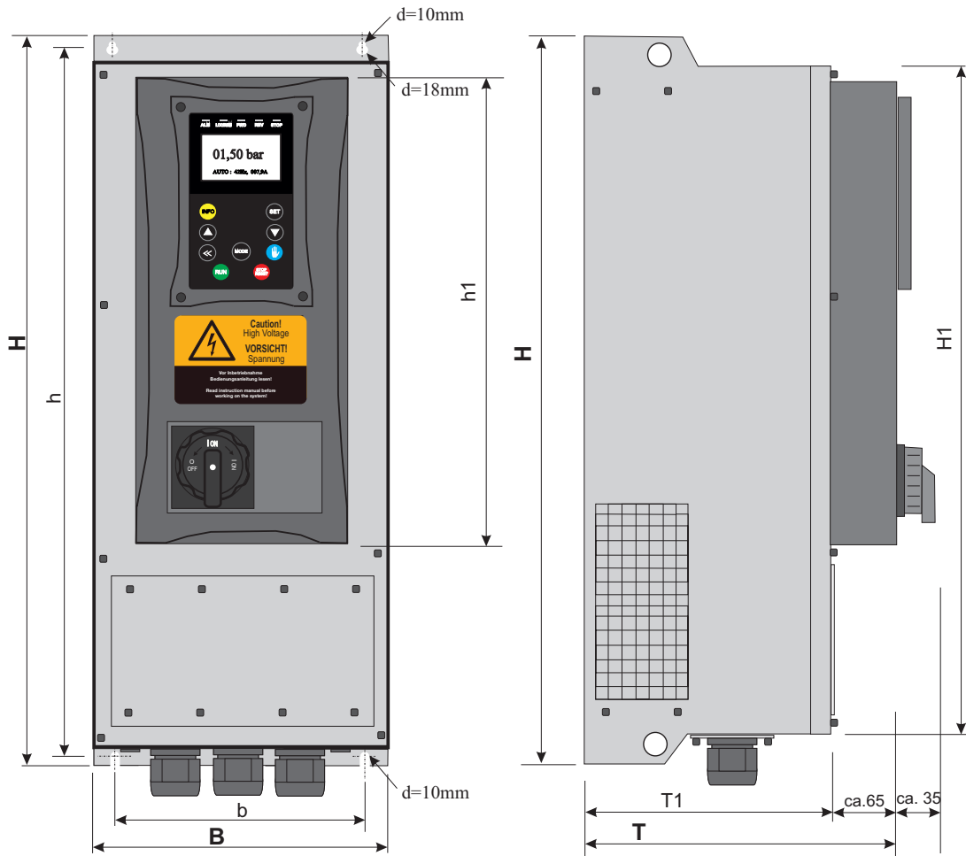
Single regulator with repair switch, MARE regulator version 2 size 3 + 4,
